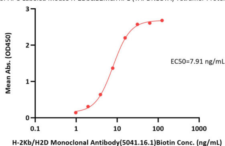
APC-Labeled Mouse H-2Db&B2M&TRP1 (TAPDNLGYA) Tetramer Protein ELISA 0.1 µg of APC-Labeled Mouse H-2Db&B2M&TRP1 (TAPDNLGYA) Tetramer Protein per well
